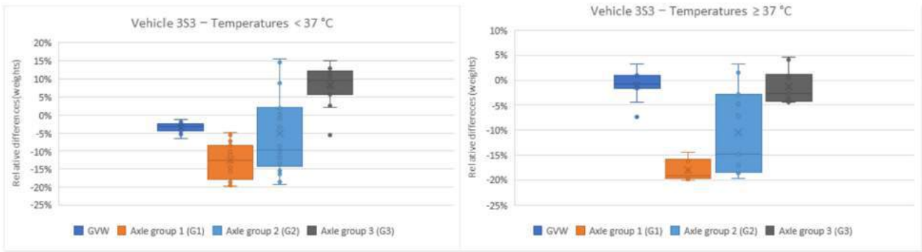
Figure 7. Box-plots of the relative differences of weight measurements by GVW and axles groups—articulated truck (353), six axles and three groups of axles—Section A02.
